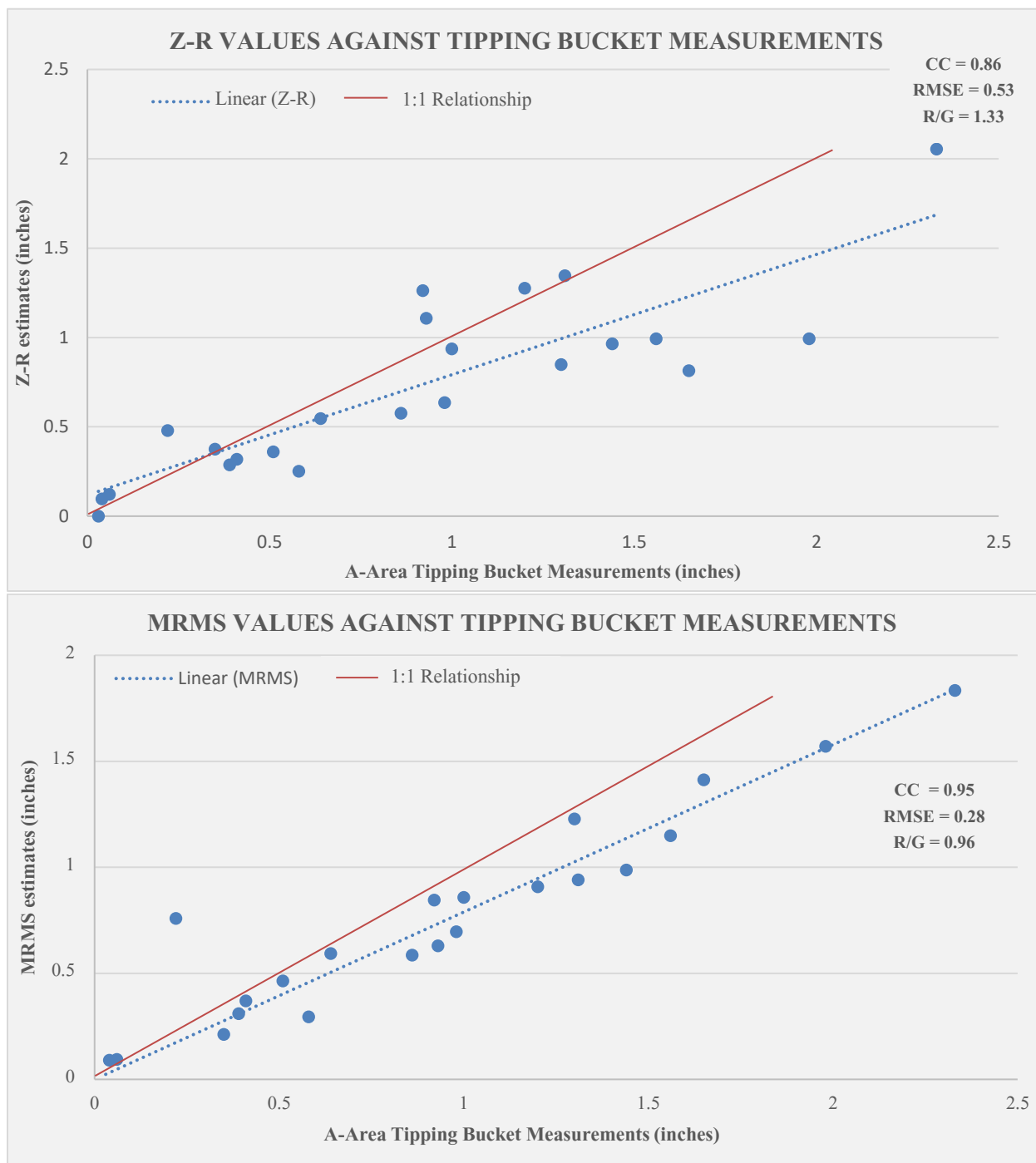
Figure 3-2. Radar Derived Values Against Tipping Bucket Measured 24-hr Rainfall Totals (continued)
