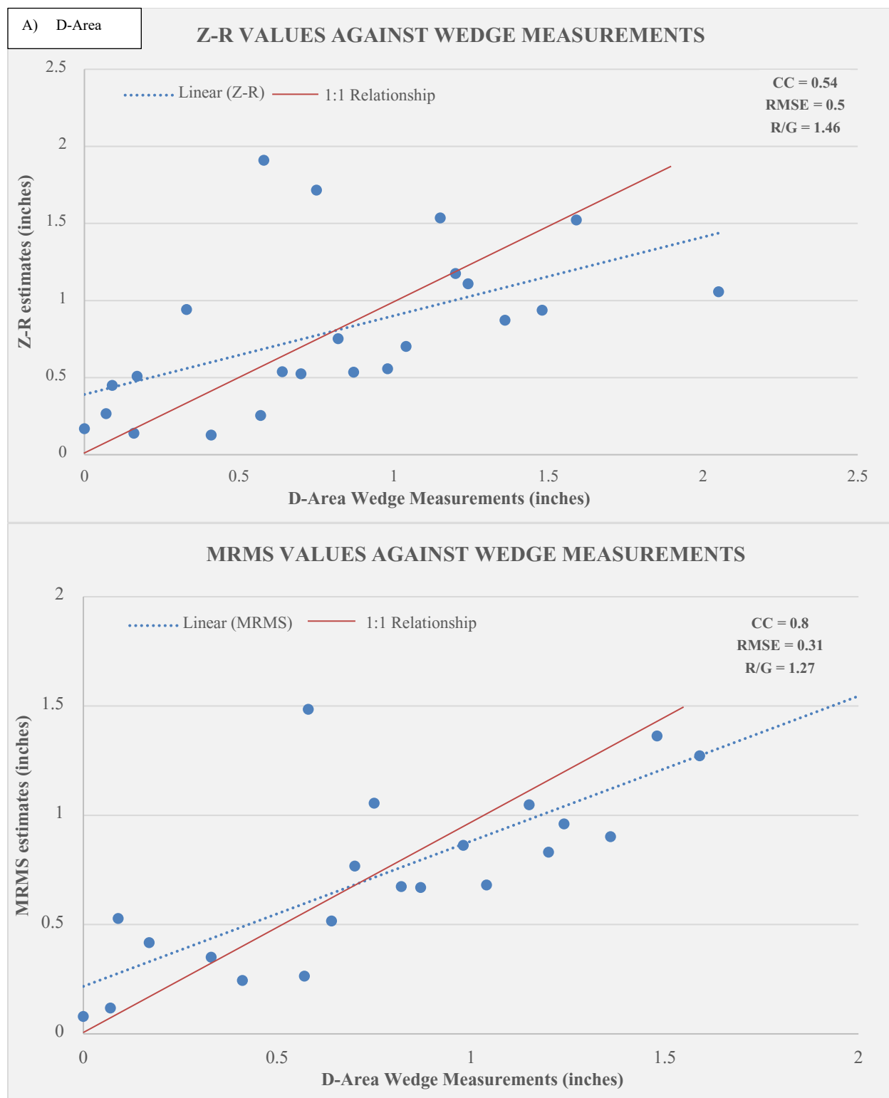
Figure 3-1. Radar Derived Values Against Wedge Measured 24-hr Rainfall Totals
