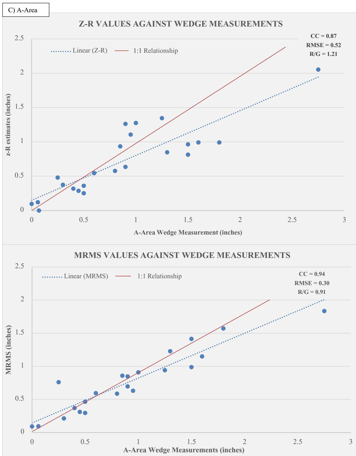
Figure 3-1. Radar Derived Values Against Wedge Measured 24-hr Rainfall Totals ( continued )
