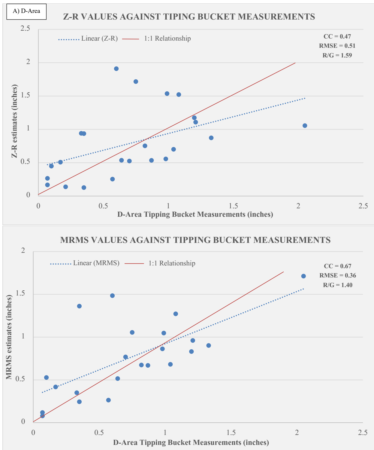
Figure 3-2. Radar Derived Values Against Tipping Bucket Measured 24-hr Rainfall Totals
