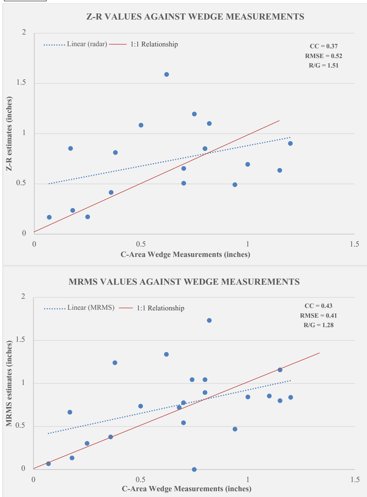
Figure 3-1. Radar Derived Values Against Wedge Measured 24-hr Rainfall Totals (continued)
