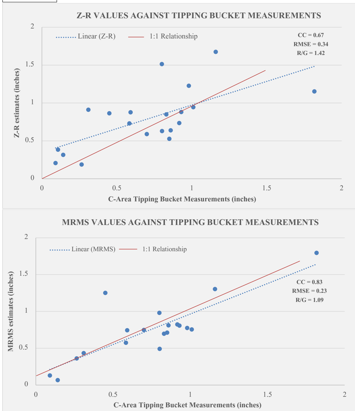
Figure 3-2. Radar Derived Values Against Tipping Bucket Measured 24-hr Rainfall Totals (continued)
